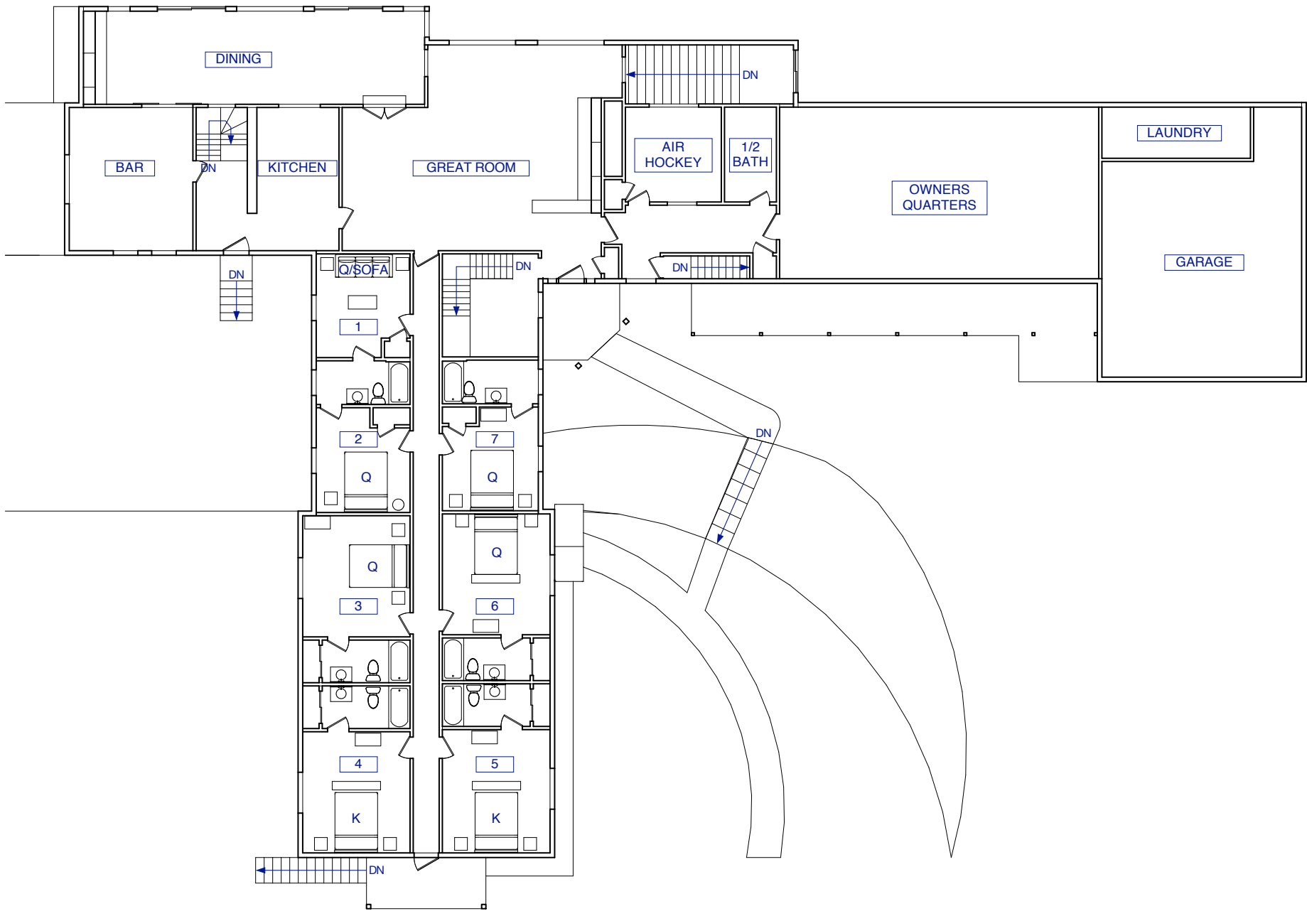
1 First Floor Plan 1/16" = 1'-0"
